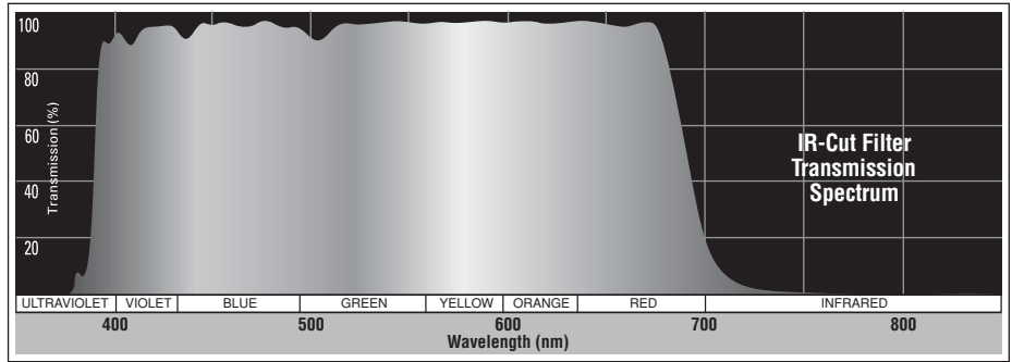
IR-Cut Filter Transmission Spectrum
