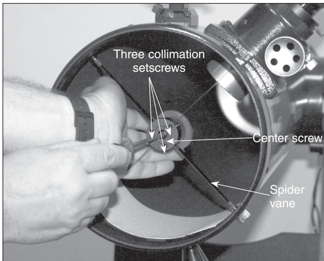
Figure 4. To center the secondary mirror under the focuser, hold the mirror holder in place with one hand while adjusting the center bolt with a Phillips screwdriver. Do not touch the mirror's surface! Adjust the tilt of the secondary mirror with the three collimation setscrews surrounding the center screw of the secondary mirror housing.
