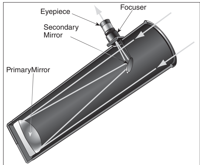
Figure 1. This diagram illustrates the Newtonian reflector's optical components. Aligning and centering these components is required for sharp, crisp images.
