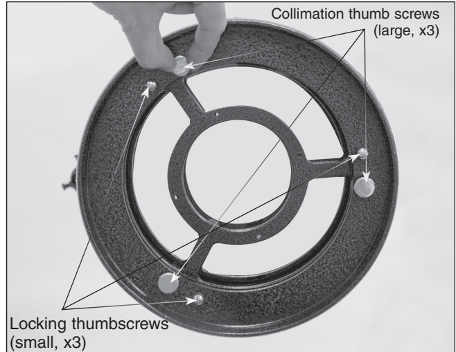
Figure 5. The three small thumbscrews that lock the primary mirror in place must first be loosened before any adjustments can be made. Then the tilt of the primary mirror can be adjusted by turning one or more of the three larger thumbscrews.
