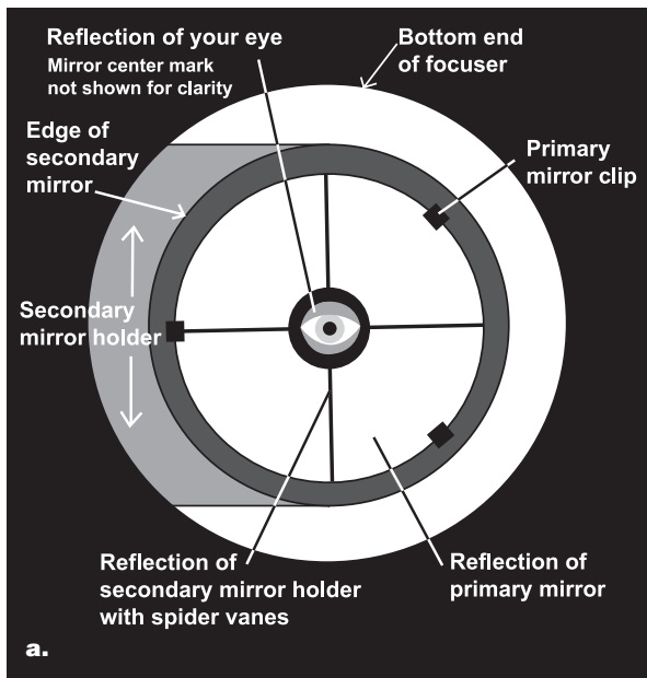
Figure 2. Collimating the optics. (a) When the mirrors are properly aligned, the view down the focuser drawtube should look like this. (b) With the collimation cap in place, if the optics are out of alignment, the view might look something like this. (c) Here, the secondary mirror is centered under the focuser, but it needs to be adjusted (tilted) so that the entire primary mirror is visible. (d) The secondary mirror is correctly aligned, but the primary mirror still needs adjustment. When the primary mirror is correctly aligned, the “dot” will be centered, as in (e).
