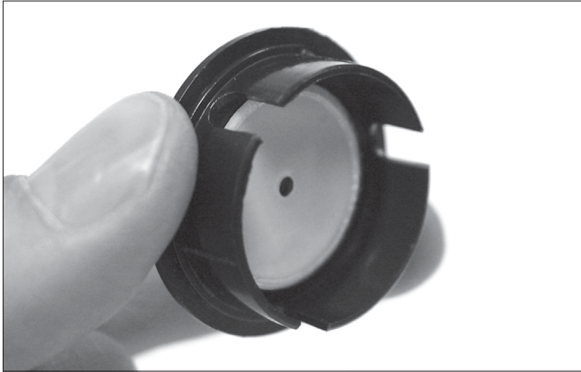
Figure 3. The quick collimation cap, which features a reflective surface on its underside, helps in centering reflections of the optics in the focuser during the collimation process.
