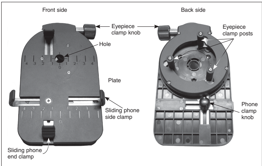
Figure 3. Parts of the SteadyPix EZ
