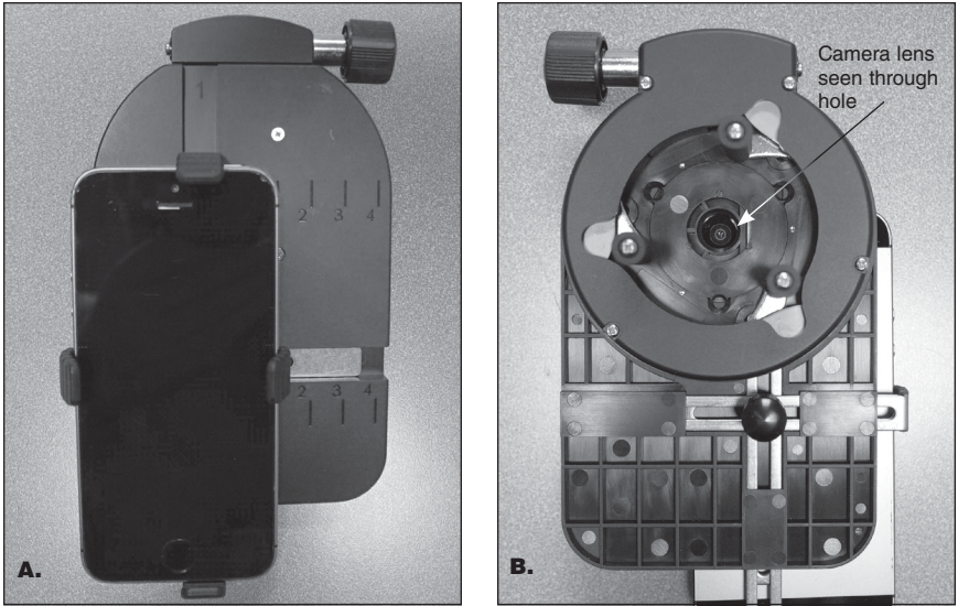
Figure 4. Center the phone's camera lens in the hole in the SteadyPix EZ's plate.
