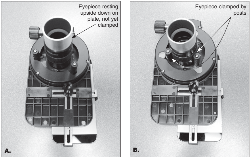
Figure 5. A) Place the eyepiece upside down on the SteadyPix as shown, then B) rotate the eyepiece clamp knob clockwise until the three clamp posts grip the eyepiece housing firmly.
