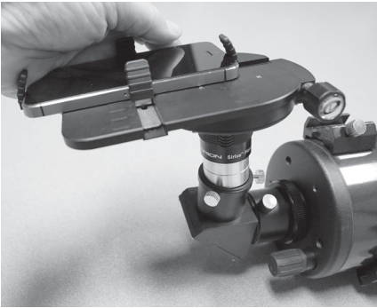
Figure 6. Insert the eyepiece with SteadyPix and phone attached into the star diagonal and secure it tightly with the thumbscrews. Before doing this be sure that the diagonal is tightly secured in the telescope’s focuser!
